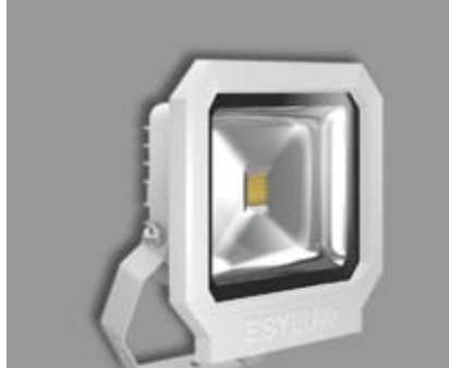
3216495.* Silber Metallic EEK: A 18 W, LED 4000 K, 710 lm H 120 L 210, B 130 € 117,80
